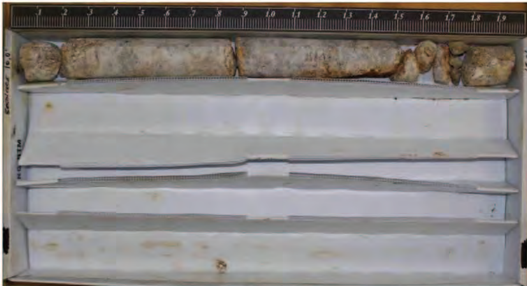
Boring EB1-B – Box 1 of 1
